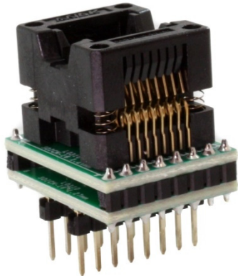
Image 1: Top View of Socket Adapter
