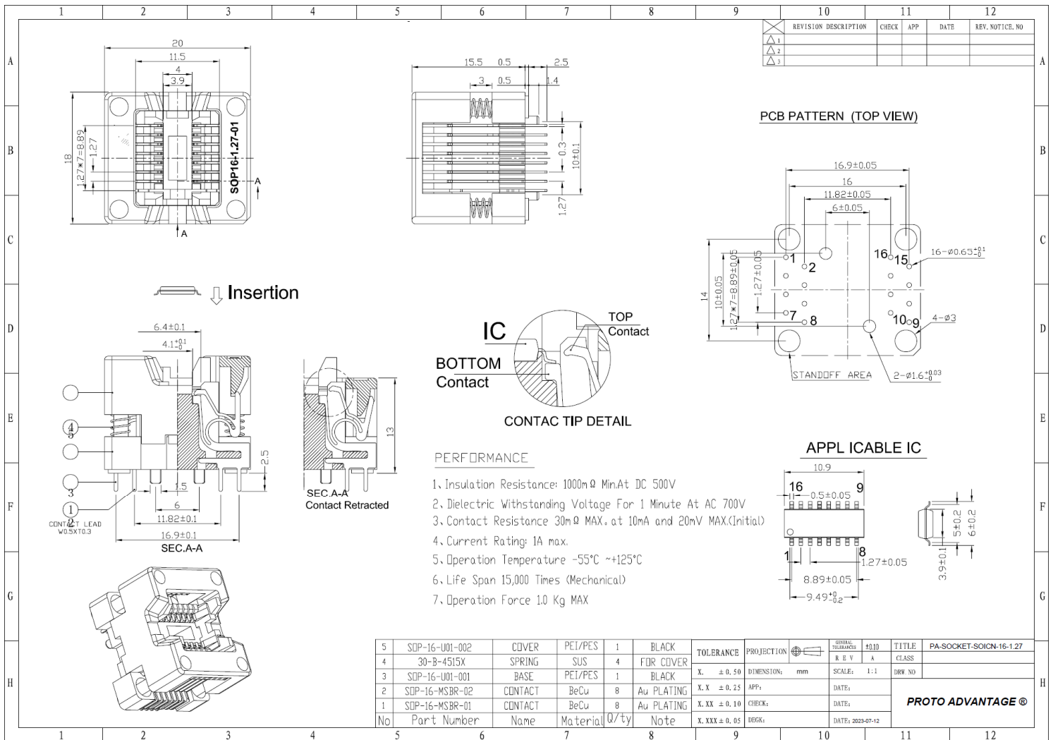
Image 3: Proto-Advantage PA-SOCKET-SOICN-16-1.27 Socket Drawing
