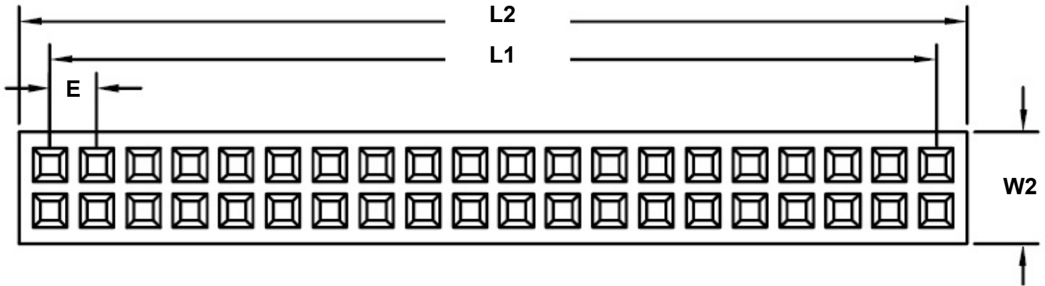
Recommended PCB Hole Layout
